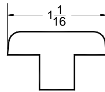
LOUVER MULLION
